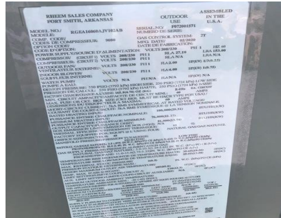
Figure 1.4 (Example picture of nameplate of HVAC unit)
