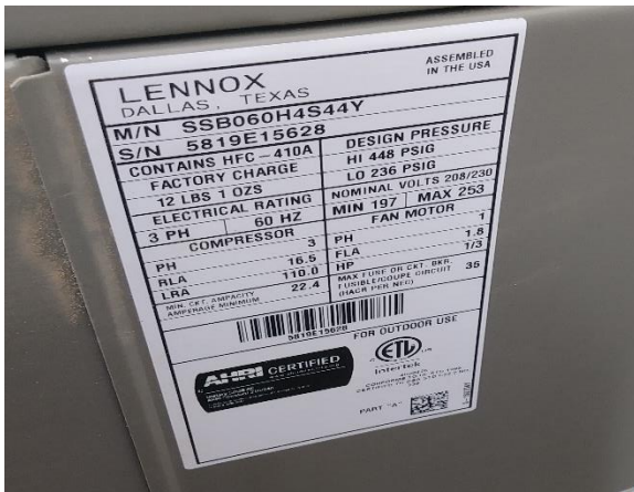
(Figure 1.7 Example picture of name plate of HVAC unit)
